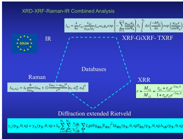
a): A XRF-GiXRF-QTA-RSA-QMA combined analysis of an \text{In}_2\text{O}_3/\text{Ag}/\text{In}_2\text{O}_3 stack, b): Implementation of more spectroscopic techniques within Combined Analysis, as envisioned in the EU SOLSA project
