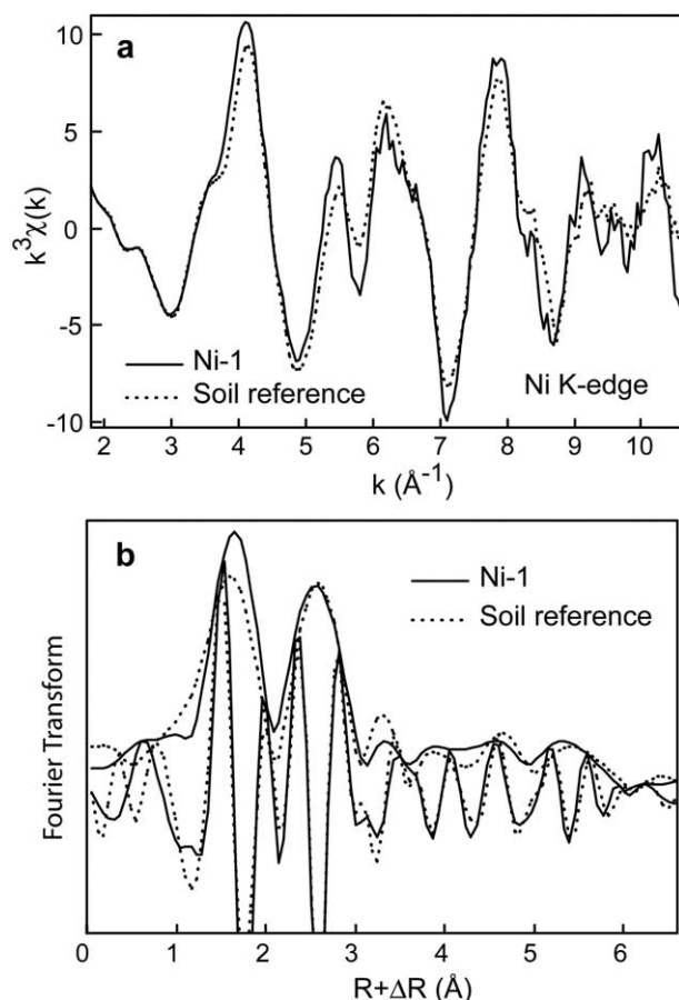
Fig. 14. Ni K-edge \mu -EXAFS collected at spot 1 and Fourier transform (Ni-1) compared to reference data in which Ni is substituted for Mn in the manganese layer of a soil lithiophorite (after Manceau et al., 2002b).
