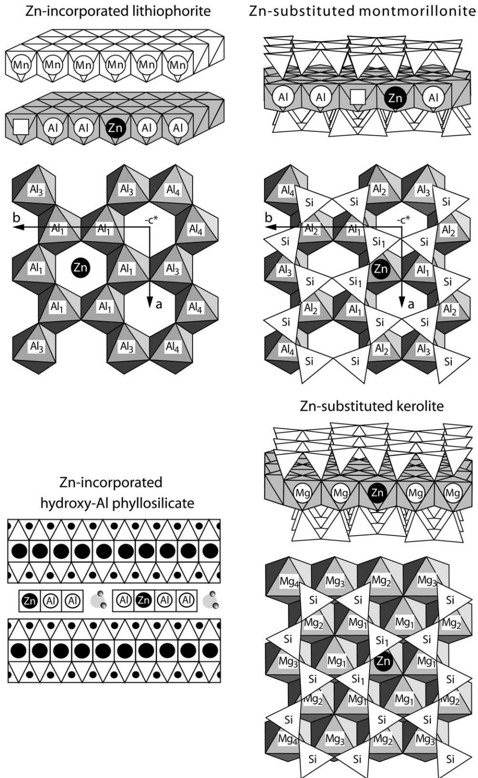
Fig. 1. Schematic representation of the site occupancy of Zn in lithiophorite, Zn-substituted montmorillonite, Zn-substituted kerolite, and hydroxy-Al phyllosilicate.
