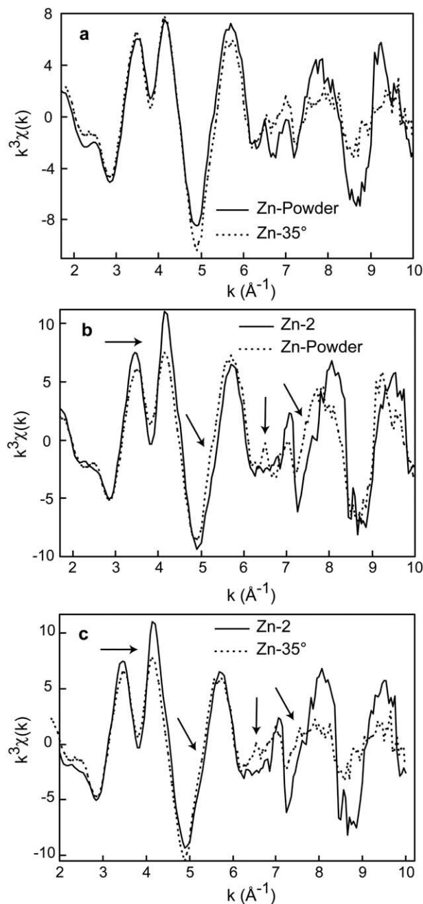
Fig. 16. (a) Zn K-edge EXAFS of an homogeneous powder from 20 Fe-Mn and Fe mottles (Zn-Powder spectrum) compared to that of the <0.2 \mu\text{m} soil fraction (Zn-35°). (b,c) Comparison of the two previous spectra with the \mu -EXAFS spectrum at spot 2 (Zn-2, lithiophorite). Spectral differences are pointed with arrows.
