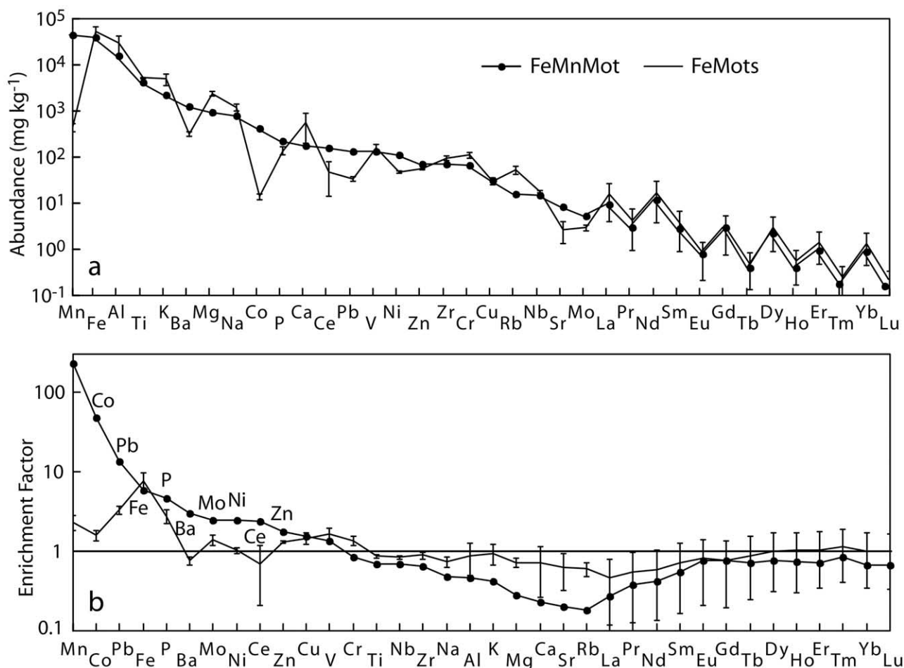
Fig. 2. Concentration of major and trace elements in the four ferruginous mottles and in the ferromanganiferous mottle (a), and enrichment factor (EF) for each element relative to the soil matrix (b). EF is defined as the ratio of the element concentration in mottle over the element concentration in the surrounding soil (Ahrens et al., 1967). The vertical bars are the standard variations calculated from the analyses of the four Fe mottles.
