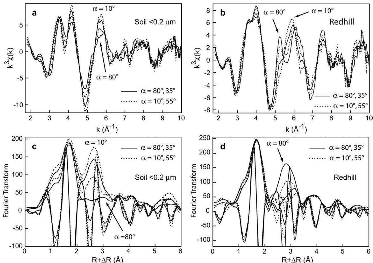
Fig. 18. Polarized EXAFS and Fourier transforms from the <0.2 \mu\text{m} soil fraction and the Redhill montmorillonite reference.
