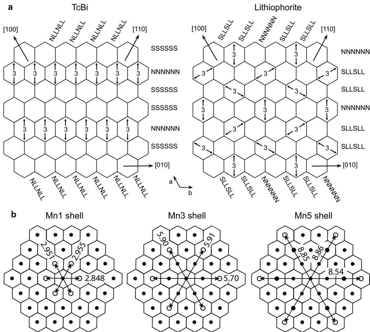
Fig. 11. (a) Schematic representation of the distribution of \text{Mn}^{3+} and \text{Mn}^{4+} cations in the manganese layer of triclinic birnessite (TcBi) and lithiophorite. (b) Mn-Mn distances for the first (Mn1), third (Mn3), and fifth (Mn5) Mn shells in triclinic birnessite (Lanson et al., 2002a). These shells have their EXAFS contribution reinforced by multiple scattering effect owing to the alignment of Mn atoms.
