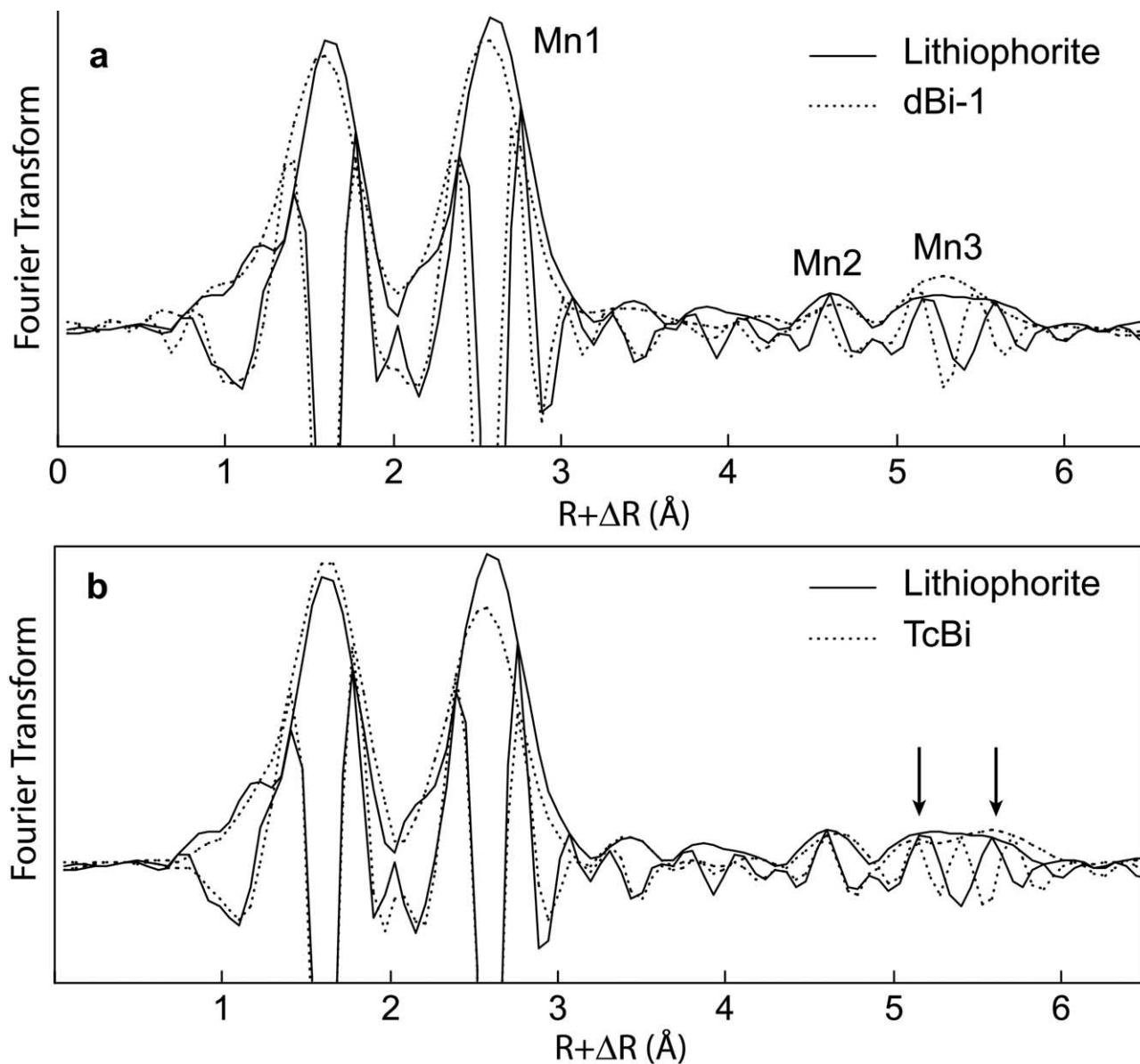
Fig. 12. Modulus and imaginary part of the Fourier transform for synthetic lithiophorite compared to those of hexagonal birnessite with only \text{Mn}^{4+} and no interlayer Mn (dBi-1) and triclinic birnessite with 31% \text{Mn}^{3+} and no interlayer Mn (TcBi). The two arrows show the splitting of the Mn-Mn distances in the third Mn shell of lithiophorite and triclinic birnessite.
