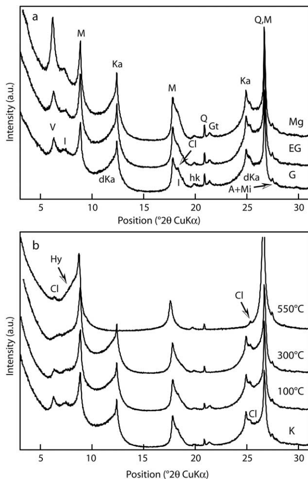
Fig. 3. XRD patterns collected on oriented preparations of the <0.2\text{-}\mu\text{m} soil size fraction. (a) Mg-saturated mount in the air-dried state (Mg) and after ethylene glycol (EG) and glycerol (G) solvation. (b) K-saturated mount (K) after ex situ thermal treatment. Cl: chlorite; M: illite/mica; Ka: ordered kaolinite; dKa: disordered kaolinite; V: vermiculite; I: interstratified illite/mica-vermiculite; A: albite; Mi: microcline; Gt: goethite; Q: quartz; Hy: Hydroxy-Al vermiculite.
