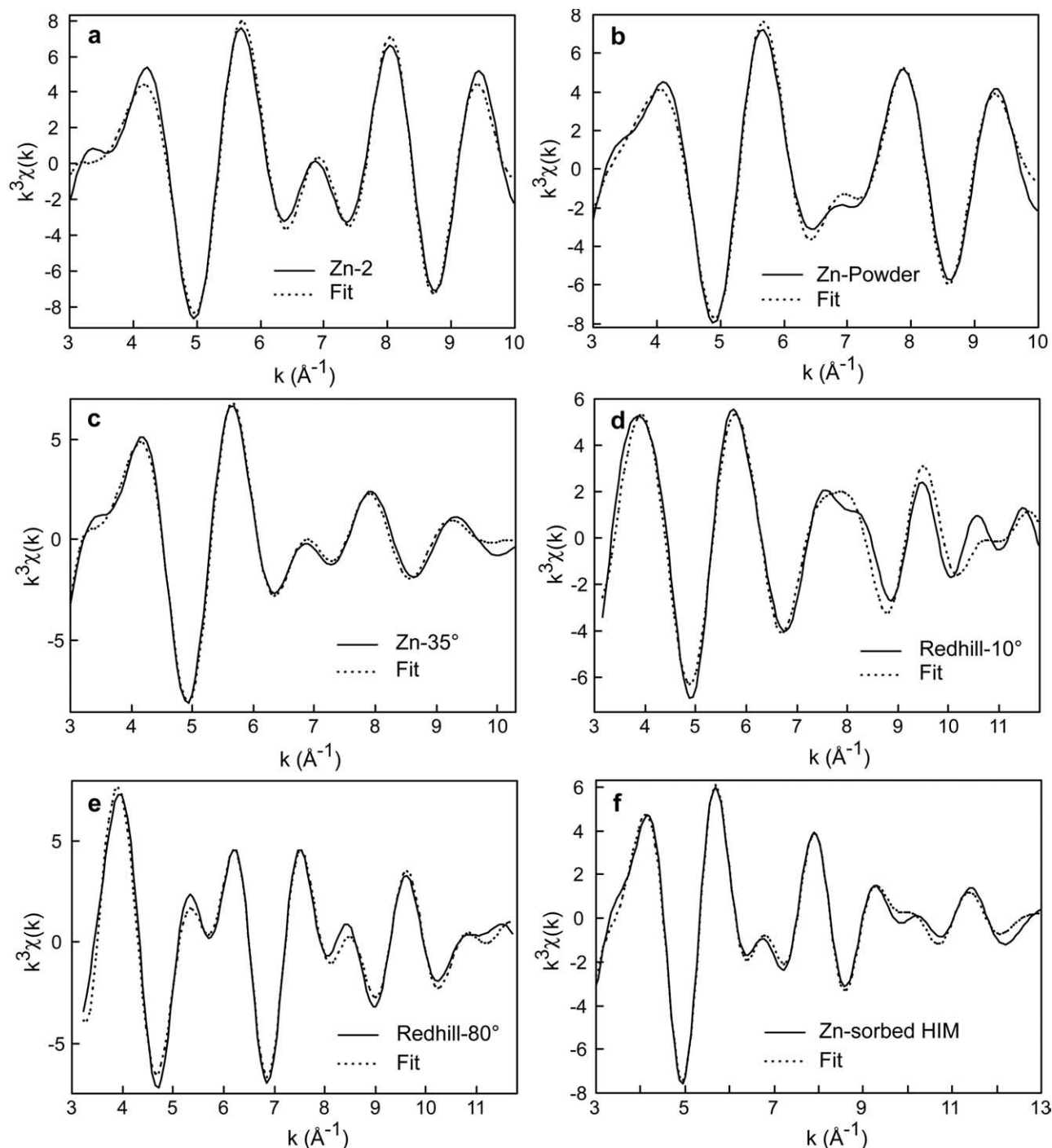
Fig. 19. Inverse Fourier transforms of the first and second RSF peaks, with spectral simulations, for the Zn data at spot 2 (Zn-2), the sample powder (Zn-Powder), the <0.2 \mu\text{m} soil fraction at \alpha = 35^\circ (Zn-35°), the Redhill montmorillonite ( \alpha = 10^\circ and 80^\circ ), and the Zn-sorbed hydroxy-Al phyllosilicate (Zn-sorbed HIM).
