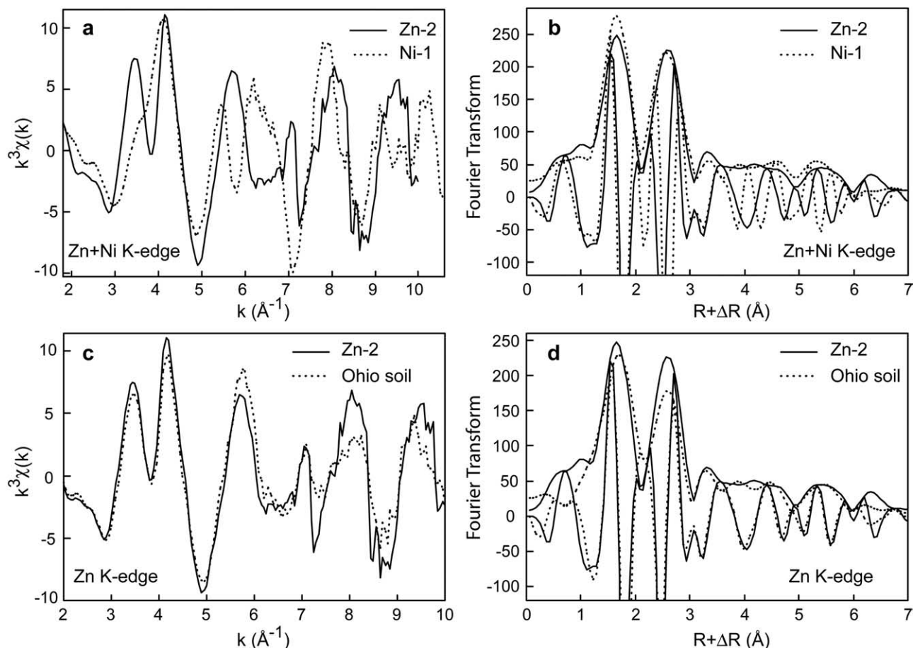
Fig. 15. (a,b) Ni (Ni-1) and Zn (Zn-2) K-edge \mu -EXAFS spectra and Fourier transforms of the soil sample. (c,d) Comparison of data obtained for the paddy soil from Taiwan and the fragipan horizon from the Ohio River basin studied by Manceau et al. (2004).
