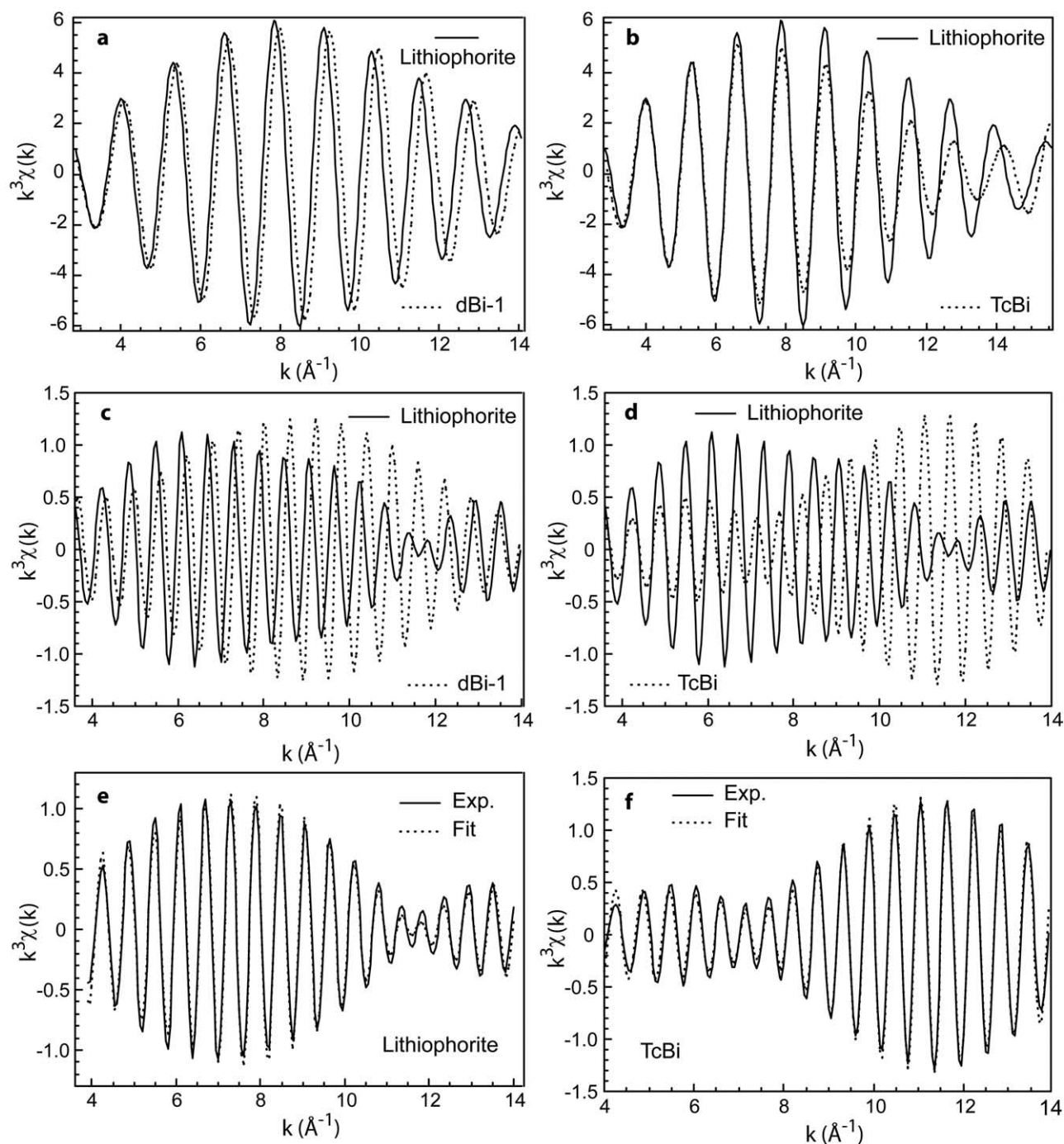
Fig. 13. Inverse Fourier transform of the synthetic lithiophorite, dBi-1 and TcBi data in the [2.1–3.1 Å] interval (Mn1 shell) (a,b), and in the [4.9–5.9 Å] interval (Mn3 shell) (c,d) with spectral simulations (e,f). In (e,f), the data are in solid lines, and the models in dotted lines.
