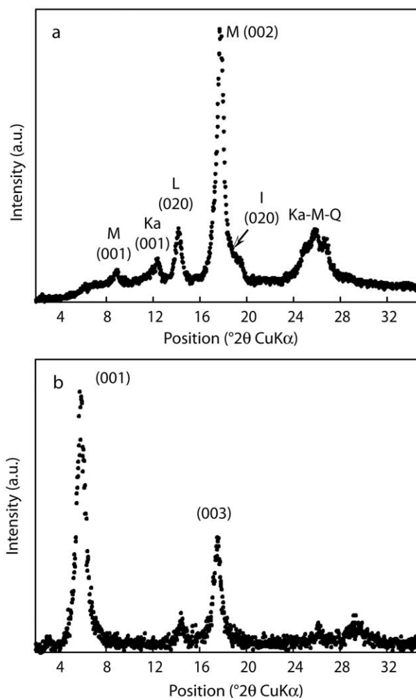
Fig. 4. XRD diagrams for the textured <0.2\text{-}\mu\text{m} soil clay fraction (a) and the textured <2\text{-}\mu\text{m} fraction of Redhill montmorillonite (b). M: mica; Ka: kaolinite; L: lepidocrocite; I: interstratified illite/mica-vermiculite; Q: quartz.
