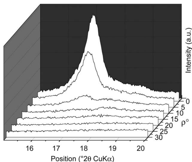
Fig. 5. Pseudo 3D diagram of the soil clay film centered on the 002 reflections of mica and illite/mica-vermiculite. The pseudo axis varies from \rho = 0^\circ (back) to 30^\circ (front) by steps of 5^\circ .
