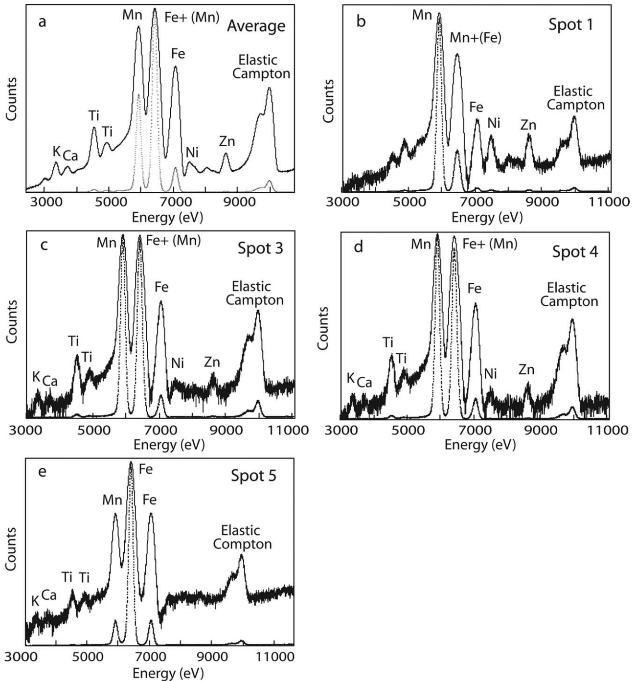
Fig. 8. X-ray fluorescence spectrum averaged over all pixels from the coarse map (i.e., taken while recording the map) (a), and XRF spectra from selected spots on the \mu -SXRF maps (b-e). Incident X-ray energy = 10 keV. Dotted line: linear scale; solid line: logarithmic scale.
