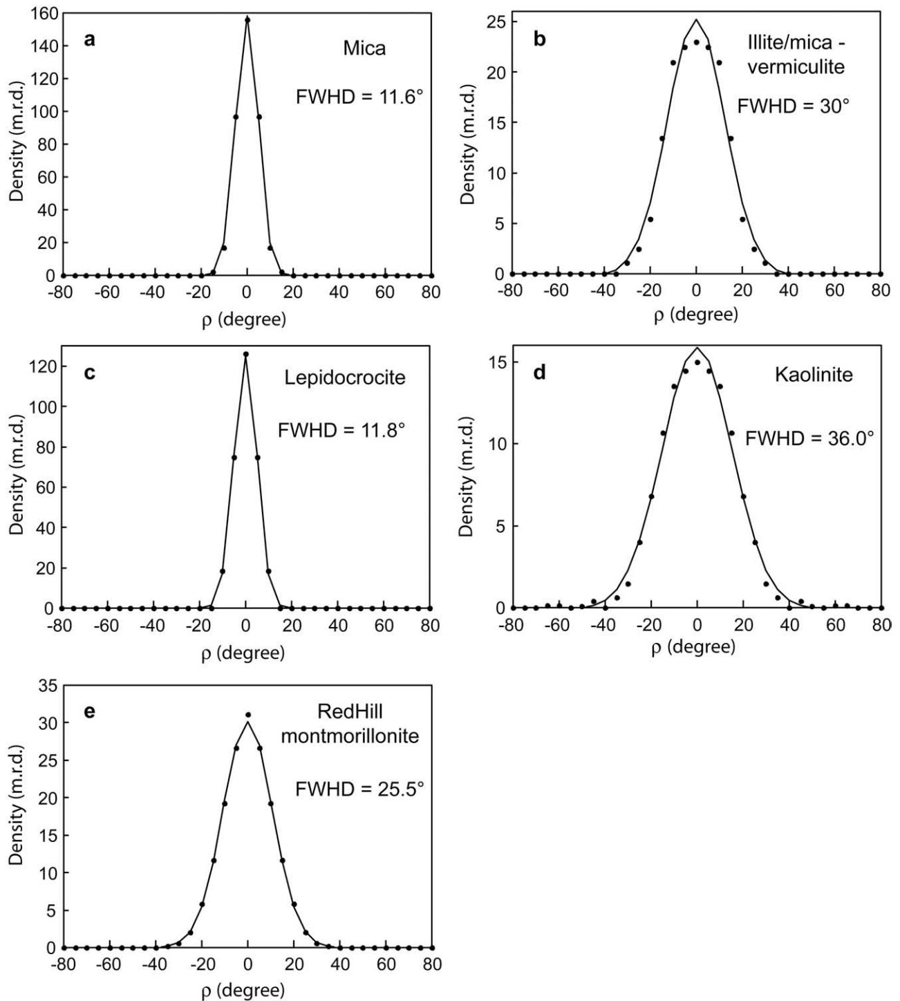
Fig. 6. Radial distribution density profiles of the 002-mica (a), 002-interstratified phase (b), 020-lepidocrocite (c), and 001-kaolinite (d) reflections for the soil clay film, and of the 001-montmorillonite reflection for the Redhill montmorillonite (e).
