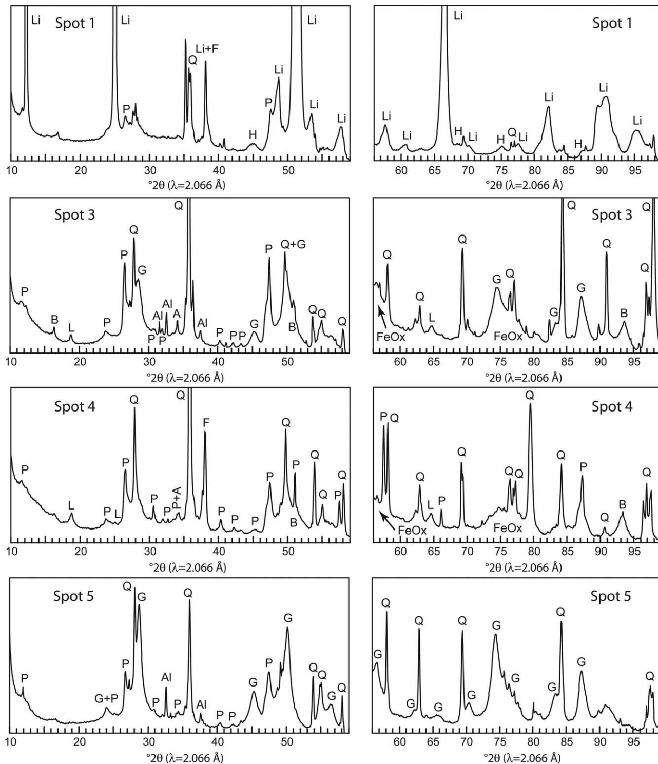
Fig. 9. One-dimensional \mu -XRD patterns ( \lambda = 2.066 \text{ \AA} ) from selected spots on the \mu -SXRF maps obtained from two-dimensional patterns by integrating intensities at constant Bragg angle. A: anatase; Al: albite; B: turbostratic hexagonal birnessite (Fe-vernadite); F: feldspath; FeOx: poorly crystalline Fe (oxyhydr)oxide (Mn-feroxyhite); G: goethite; H: hematite; L: lepidocrocite; Li: lithiophorite; P: phyllosilicate; Q: quartz. The relative intensity of the hkl reflections for the coarse grains is different from the powder pattern of the same mineral species because only a few individual crystals satisfy the Bragg condition in \mu -XRD experiment.
