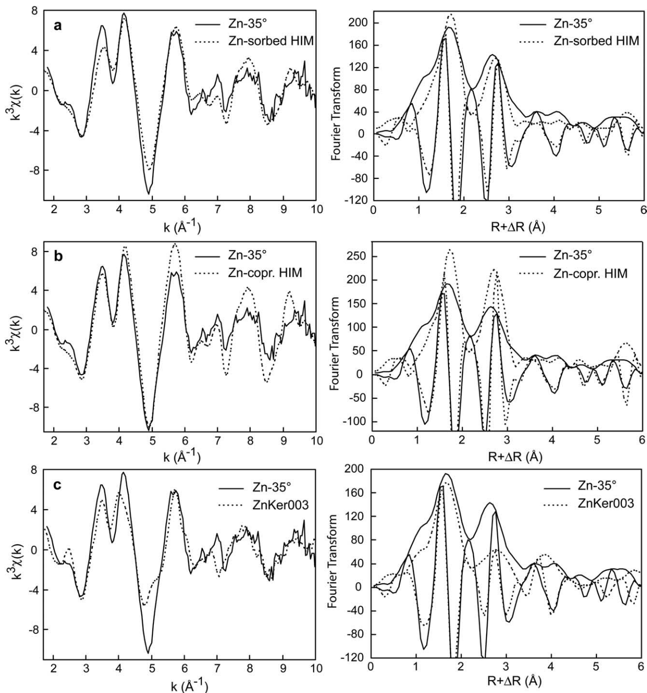
Fig. 17. Zn K-edge EXAFS spectrum from the <0.2 \mu\text{m} soil fraction (Zn-35°) compared to a selection of reference compounds: Zn-sorbed (Zn-sorbed HIM) and Zn-coprecipitated (Zn-copr. HIM) hydroxy-Al interlayered phyllosilicate, Zn-substituted kerolite (ZnKer003, \text{Zn}_{0.03}\text{Mg}_{2.97}\text{Si}_4\text{O}_{10}(\text{OH})_2 \cdot n\text{H}_2\text{O} ), natural Zn-containing montmorillonites (SAZ-1 and Redhill), and Zn-Al layered double hydroxide (LDH, \text{Zn}_2\text{Al}(\text{Kim et al.})_6[\text{CO}_3]_{0.5} ). Kerolite is used as a proxy for the general class of Zn-containing trioctahedral phyllosilicate.
