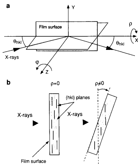
Figure 7. X-ray diffraction reflection geometry used for texture analysis. a): A \{hkl\} pole figure is measured for a fixed \theta_{hkl} , while the sample is rotated by \rho and \phi (both conserving \theta_{hkl} ). b): Side view of (a) showing how individual crystallographic planes within the film are brought to a diffraction position by a rotation of \rho .
