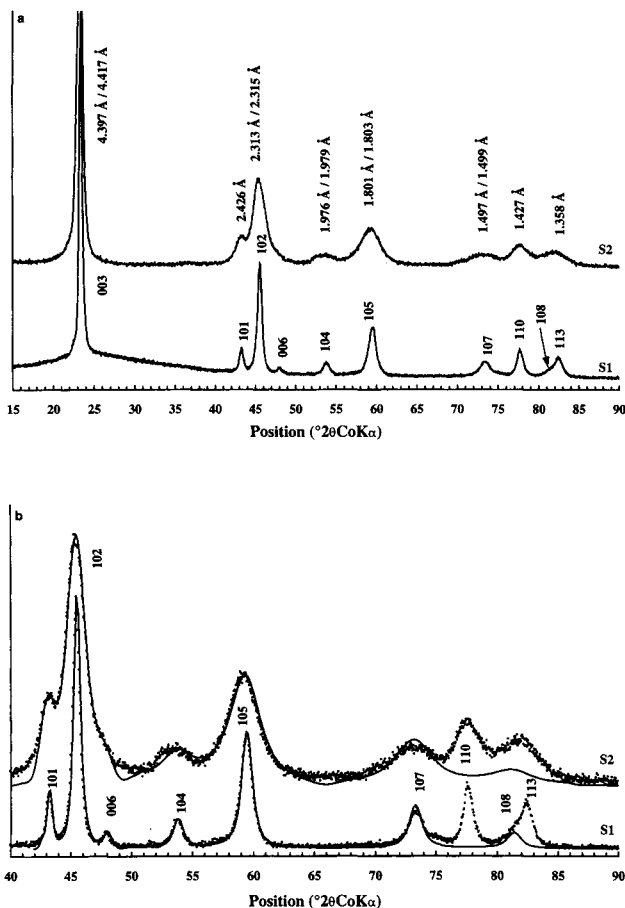
Figure 19. a) Experimental XRD pattern of synthetic CoOOH and indexing in a three-layer hexagonal unit cell (3R). a = 2.850 \text{ \AA} , c = 13.198 \text{ \AA} , \gamma = 120^\circ for S1 and a = 2.855 \text{ \AA} , c = 13.200 \text{ \AA} , \gamma = 120^\circ , for S2. When two d(hkl) values are given they refer to samples S1 and S2, respectively. b) Comparison between experimental (dots) and calculated (solid lines) XRD patterns. Only 10l lines were calculated. For S1, N_{\text{mean}} = 3 , N_{\text{max}} = 12 , \Phi = 270 \text{ \AA} , W_R = 0\% , and the proportion of Co vacancies is 15%. For S2, N_{\text{mean}} = 2 , N_{\text{max}} = 5 , \Phi = 100 \text{ \AA} , W_R = 45\% , and the proportion of Co vacancies is 8%. N is the number of 3-layer units stacked coherently.
