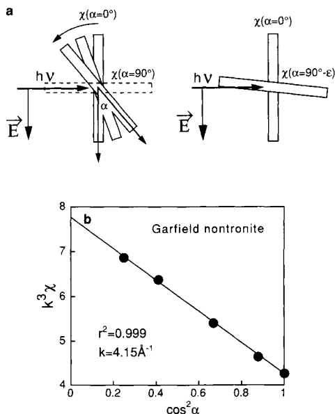
Figure 6. a) Measurement of angular spectra in transmission mode (left) and grazing incidence (right). In both cases, the film is rotated around an axis perpendicular to both the beam direction and \vec{E} . b) Plot of k^3\chi as a function of \cos^2\alpha which confirms the expected angular dependence of EXAFS spectra.
