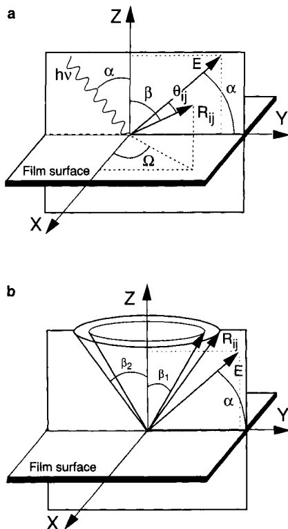
Figure 3. a) Coordinate system applicable to angular measurements on self-supporting films. XY is the film plane, and X -rays are incident on the YZ plane. \alpha is the incidence angle between E and Y , \beta is the polar angle, and \Omega the azimuthal angle of the atomic pair ij . \theta_{ij} is the angle between E and the atomic pair. b) Distribution of orientation of \beta angles of atomic pairs resulting from the misalignment of c^* axis of individual particles perpendicularly to the film surface. The disorientation is equal to \Delta\beta = \beta_2 - \beta_1 .
