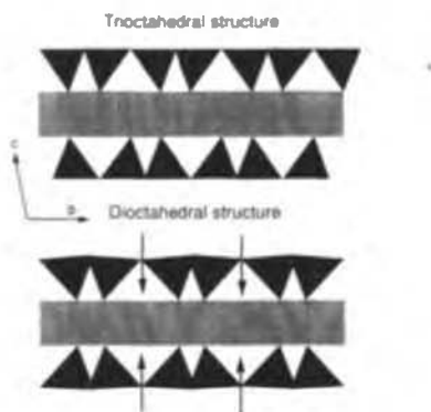
Figure 14. Representation of the biotite and nontronite structure projected down [100].
