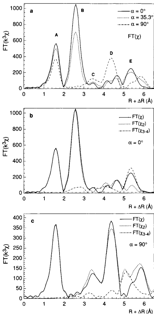
Figure 24. a) P-RSFs of FEFF spectra for \alpha = 0^\circ , 35.3^\circ , and 90^\circ . RSFs of single ( \chi_2 ), multiple ( \chi_{3-4} ) and total ( \chi ) scattering-paths for \alpha = 0^\circ (b) and \alpha = 90^\circ (c).
