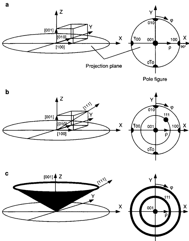
Figure 8. a) Definition of the projection plane for a pole figure, with respect to sample coordinates (left) and schematic \{001\} pole figure in the case of a single crystal with cubic symmetry with main axes oriented parallel to the sample frame (right). b) [111] crystalline direction for the single crystal (left) and its localization on the pole figure frame (right), not shown here are the other equivalent crystal directions for a cubic crystal symmetry. c) Same as in b) for a set of crystals randomly oriented around Z with [001] directions parallel to Z ( \langle 001 \rangle fiber texture), the pole figure exhibits rings for all directions at the corresponding \rho value.
