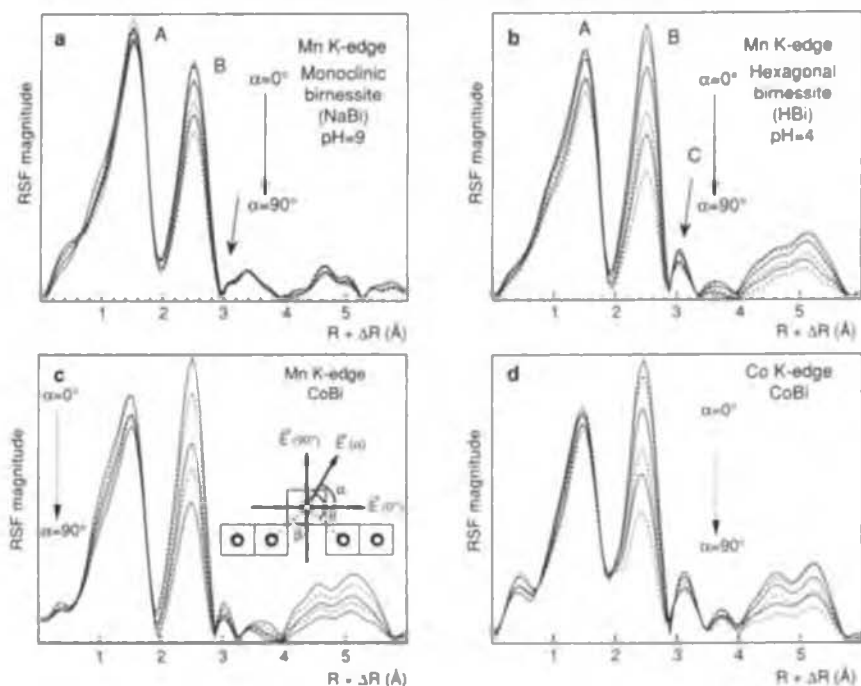
Figure 17. Polarized RSFs for NaBi (a), HBi (b), and CoBi (c,d). The 90° spectra have been calculated as discussed in the text.
