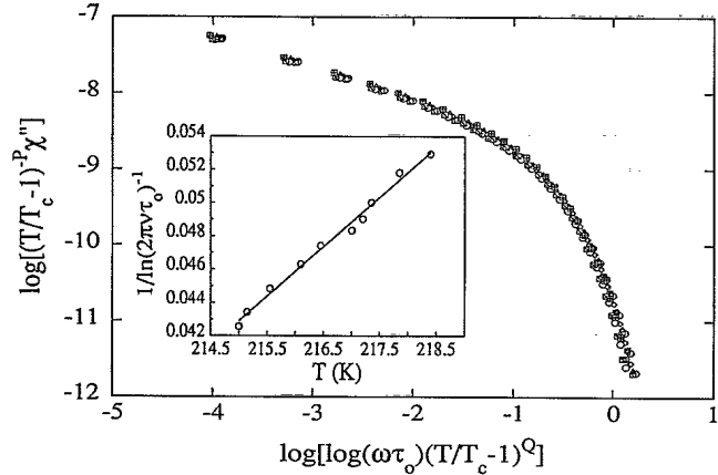
FIG. 12. Activated dynamic scaling \chi'' = t^P G[-\ln(\omega\tau_0)t^Q] , with t = T/T_c - 1 ( T_c = 215.5 K), P = 1.4 , Q = 0.55 , and \tau_0 = 10^{-12} s, for seven sets of measurements of sample C with h_{ac} = 5 Oe and frequencies between 16 and 1000 Hz. Inset: Variation of the temperature of the maximum of the imaginary part of the ac susceptibility with the frequency of the ac field ( h_{ac} = 5 Oe), in a Vogel-Fulcher plot for sample C. From the linearity of this plot we obtain \tau_0 = 10^{-12} s.
