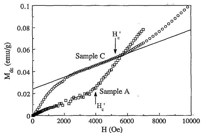
FIG. 6. First magnetization curves measured at 5 K after ZFC for samples A (squares) and C (circles). The linear fit of the saturation magnetization of sample C below H'_c is also plotted. The arrows signal H'_c (5 K) for both samples.
