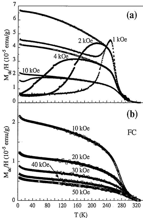
FIG. 2. M_{dc}/H vs T of sample A, (a) measured after ZFC (inferior curves) and FC (superior curves) in 1, 2, 4, and 10 kOe and (b) measured after FC in 10, 20, 30, 40, and 50 kOe.
