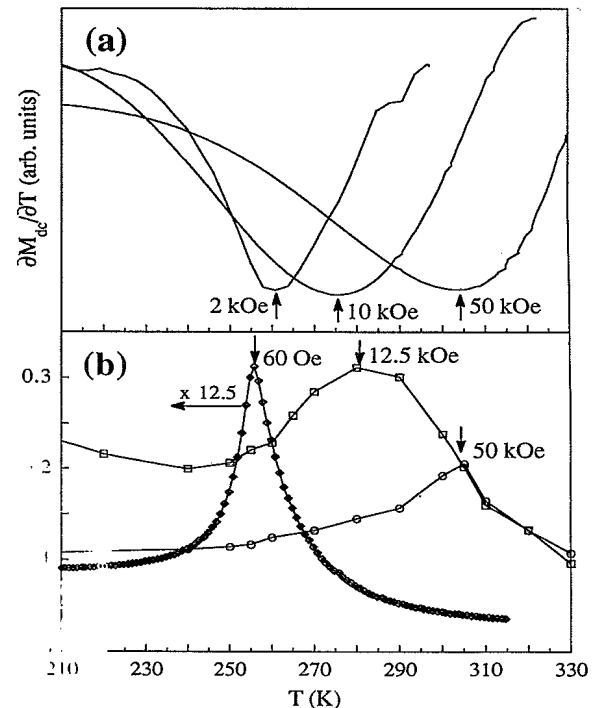
FIG. 9. (a) Derivative of the dc magnetization with temperature for sample A and fields of 2, 10, and 50 kOe. (b) Differential susceptibility versus temperature of sample A at 60 Oe, 12.5, and 50 kOe. In both cases, the arrows indicate the maxima which define the points of the WF transition.
