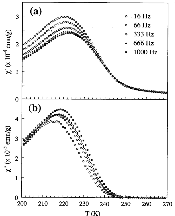
FIG. 8. Real (a) and imaginary (b) parts of the ac susceptibility of sample C, measured with h_{ac} = 5 Oe and frequencies between 16 and 1000 Hz.
