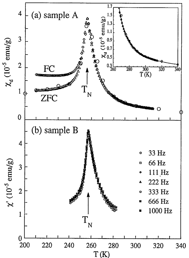
FIG. 1. (a) M_{\text{dc}}/H measured for sample A with H=60 Oe after field cooling (diamonds) and zero-field cooling (triangles). Circles correspond to the differential susceptibility \chi_d \equiv \partial M_{\text{dc}}/\partial H at low fields. Inset: Fit of the high-temperature part of the susceptibility to \chi_d(T) = \chi_0 + (D\chi_0)^2 \nu^{-1} (T - T_N)^{-\gamma} . (b) Real part of the ac susceptibility, \chi'(T) , vs temperature measured for sample B with h_{\text{ac}}=5 Oe and different frequencies between 33 and 1000 Hz.
