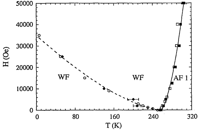
FIG. 10. Phase diagram of sample A of Y_2CuO_4 at high magnetic fields. Open squares are the inflexion points of the M_{dc}(T) curves, full squares are the maximum of the \chi_a(T) curves, and the solid line is a fit to the function H = H_0(T/T_N - 1)^{\gamma+\beta} . Circles are the irreversibility points of the M_{dc}(H) cycles and the dotted line is a fit to the law H = H_0(1 - T/T_N)^{3/2} . The irreversibility points of sample C are also plotted as full diamonds.
