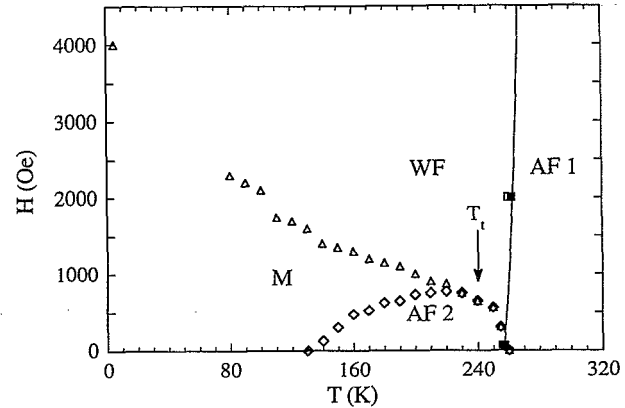
FIG. 5. Phase diagram of sample A of Y_2CuO_4 . Triangles and diamonds correspond to the critical fields H'_c and H''_c , respectively. The squares and the solid line determine the WF transition.
