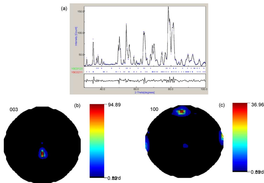
Fig. 2. (a) Rietveld refinement of the sum of the 1368 measured diagrams, allowing phase, cell parameters quantitative determinations. (b) {003} and (c) {100} pole figure showing the strong orientation of the Y123 phase with one single domain.
